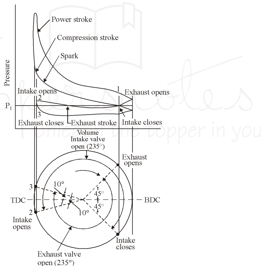
Fig. Four-stroke petrol engine valve timing diagram in relation to the pressure volume diagram
