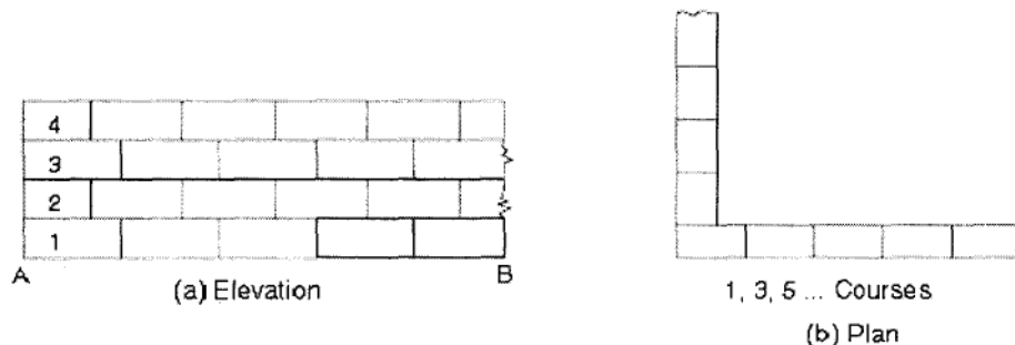
Stretcher bond
