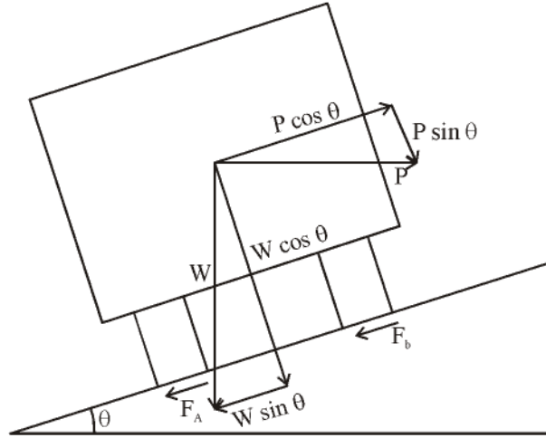
Fig. : Analysis of super-elevation
