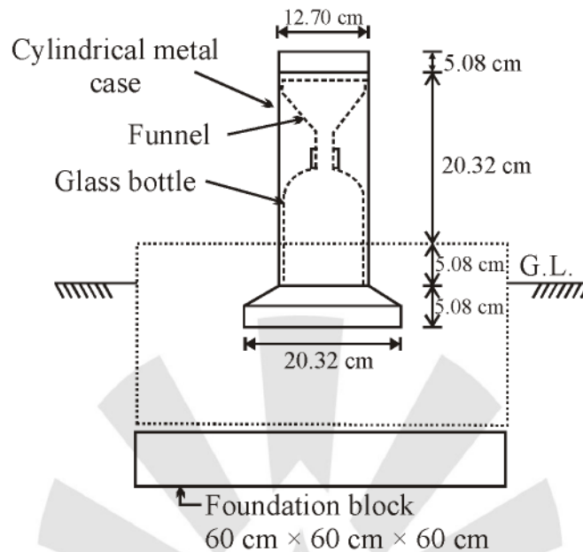
Fig. 2.1 : Symon's rain gauge
