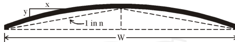
(a) Parabolic camber y = \frac{2x^2}{nW}
